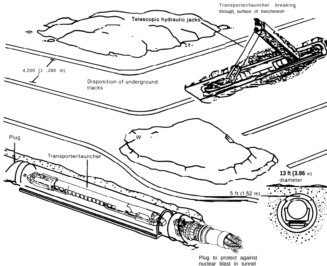
Figure 51.—Trench Layout
