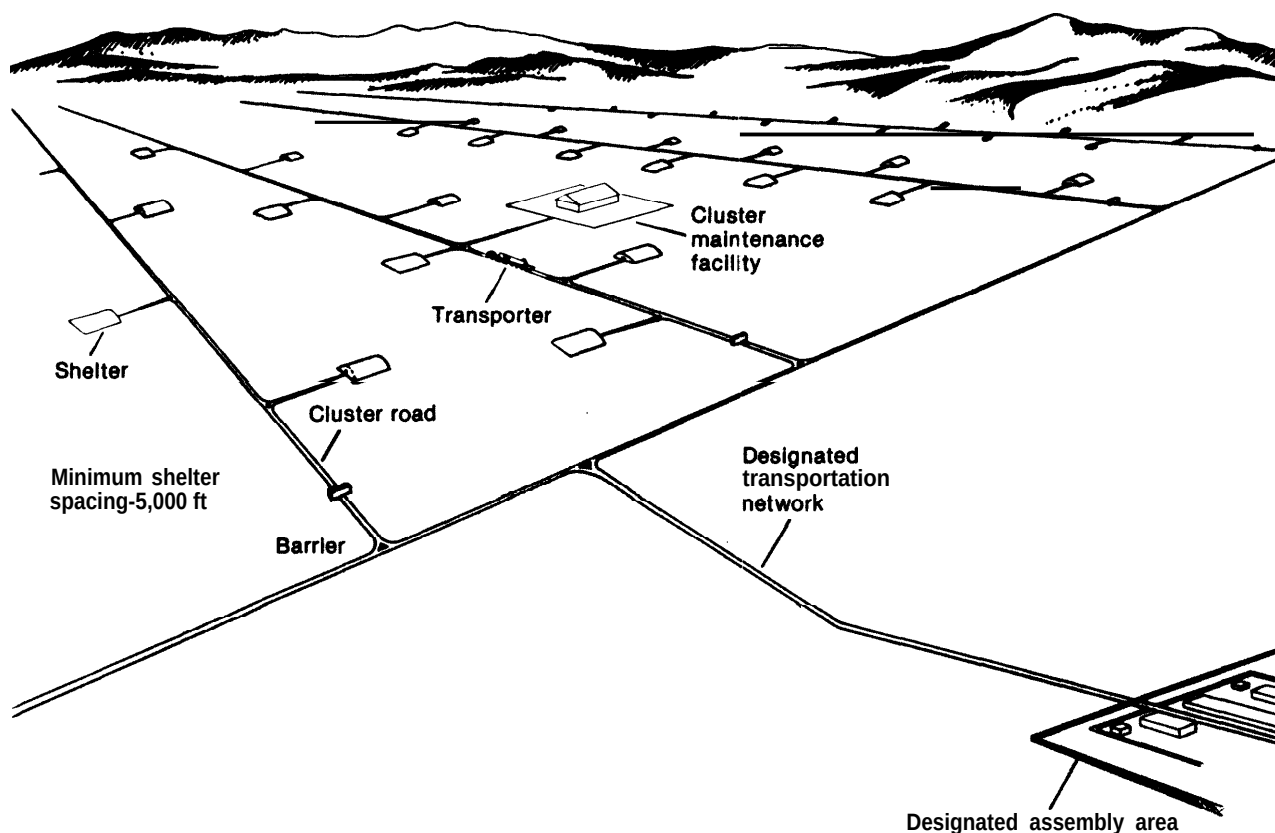
Figure 14.—System Description
