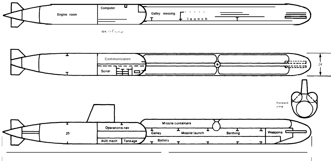
Figure 69.— MX"Carrying Diesel. Electric Small Submarine 4 (3,300 tons submerged displacement)
