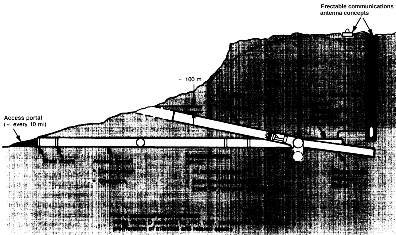
Figure 11 7.—Mesa/Tunnel Concept Section View (not to scale)
