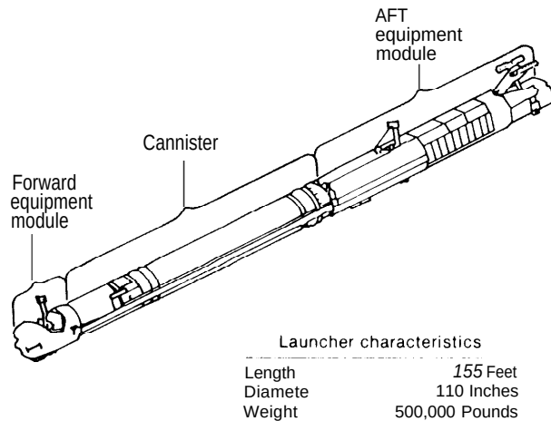
Figure 15.—Launcher
