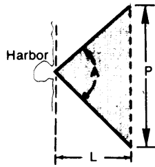
Figure 100.—Geometry of Barrier Outside a Port With Unobstructed Access to the Sea
