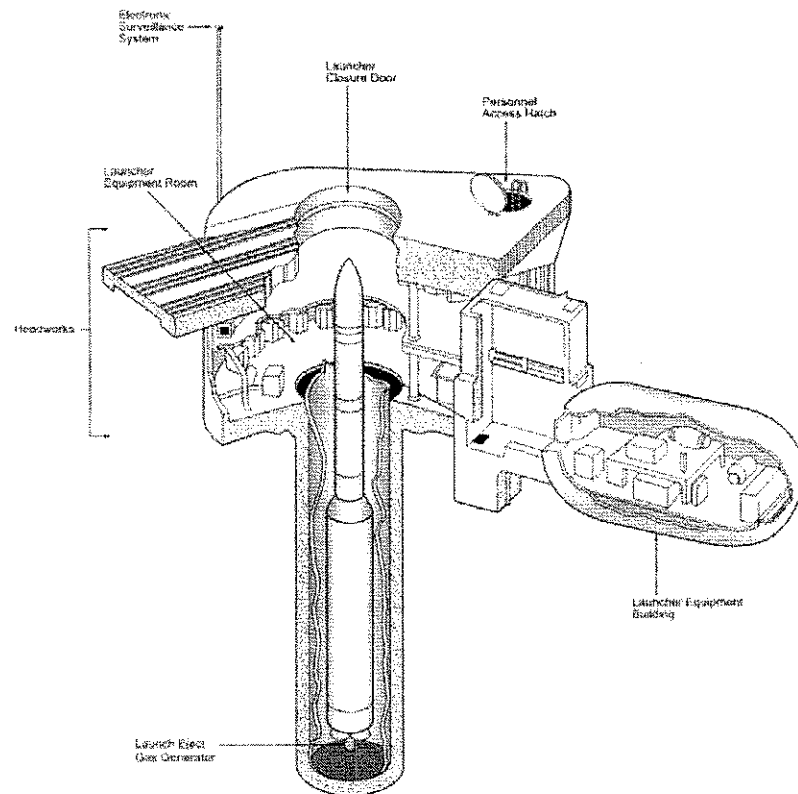
Launch Facility Schematic
